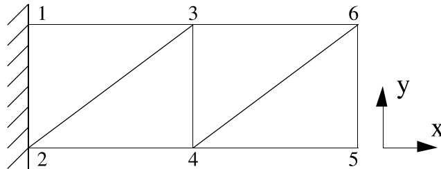
Figure 4.1: FE model.
