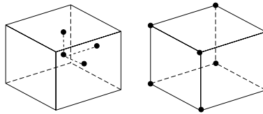
Figure 10.4: Sample experiments. a) Hypercube face center. b) Classical 2^{NP} factorial plan.
