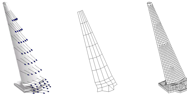
Figure 3.1: FE and wire-frame models
